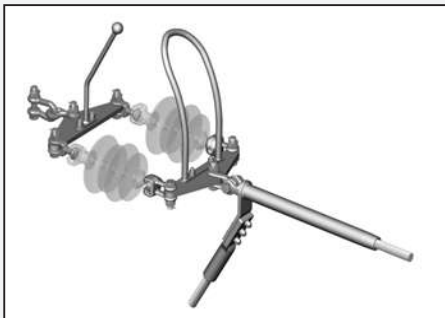
220kV DOUBLE- Tension
